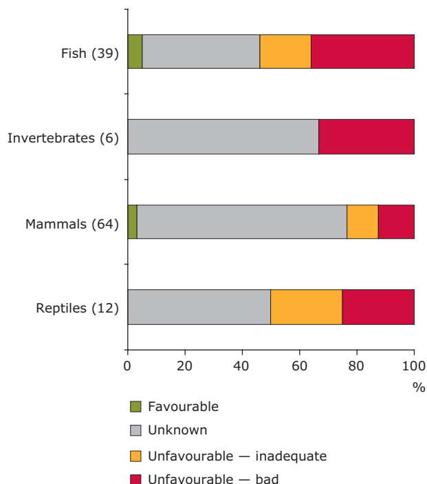
Figure 2.5 Conservation status of species of European interest in marine habitats
